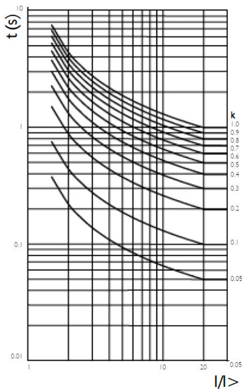
Tripping Curve Characteristics (Normal Inverse I^{3/10} ) ^
