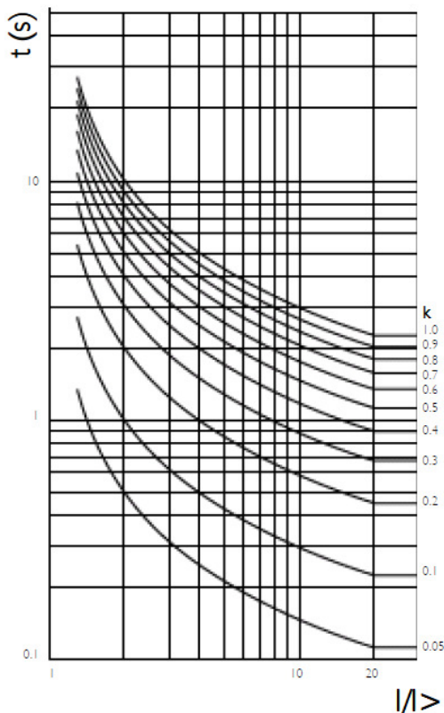
Tripping Curve Characteristics (Normal Inverse I^{3/10} ) ^
