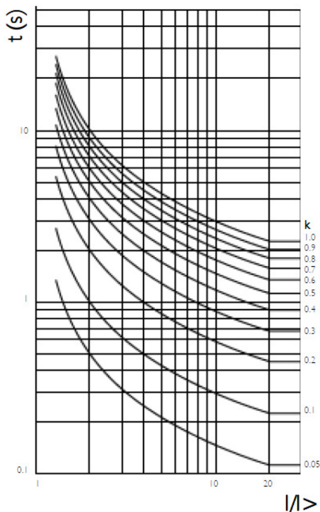
Tripping Curve Characteristics (Normal Inverse 3/10)
